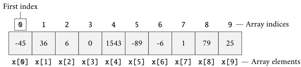
Figure 6.1. Elements of an array in C++
